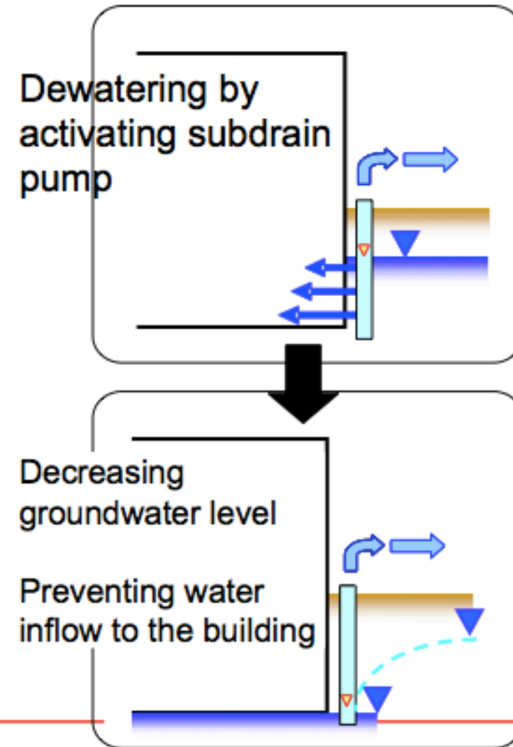
Pumping up groundwater (subdrain)
