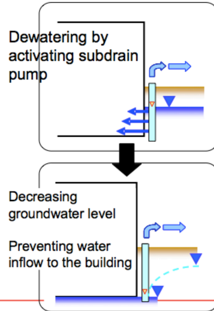
Pumping up groundwater (subdrain)
