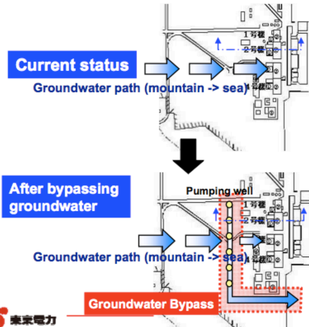
Groundwater bypass
